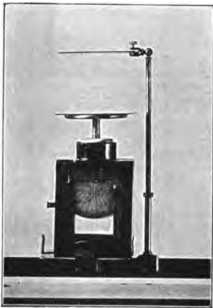
FIG. 37.—Apparatus for reducing the rapidity of the loss of electricity produced by radio-active bodies.—The radio-active substance is placed in a metal capsule placed on the plate of the electroscope, and the speed of the discharge is varied by means of a metallic blade placed at greater or lesser distance from the plate.
